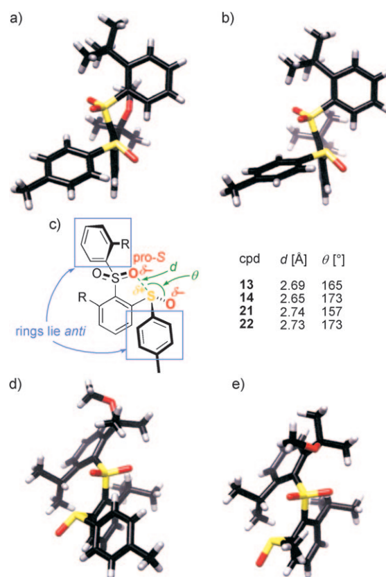
Figure 2. X-ray crystal structures of a) 13 and b) 14 , both showing the favored ( R , M ) conformation. c) Presumed governing SO 2 –SO dipole/Ar–Ar steric interaction, with values of d (distance between sulfone pro- S O atom and sulfoxide S atom) and \theta (angle formed by sulfone pro- S O, sulfoxide S, and sulfoxide O atoms) for 13 , 14 , 21 , and 22 . X-ray crystal structures of d) 21 and e) 22 , [12] both showing the favored ( S , P ) conformation.
